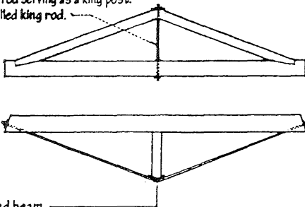
trussed beam
