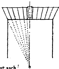
flat arch An arch having a horizontal intrados with voussoirs radiating from a center below, often built with a slight camber to allow for settling. Also called jack arch .
