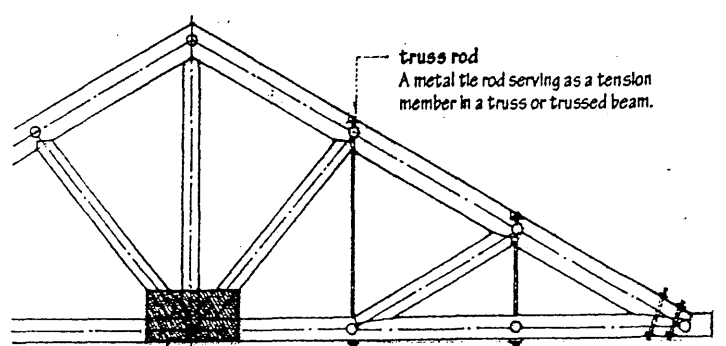
composite truss
