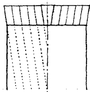
French arch A flat arch having voussoirs inclined to the same angle on each side of the center.
