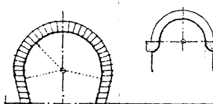
stilted arch An arch resting on imposts treated as downward continuations of the archivolts.
