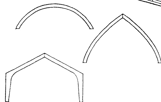
examples of glue-laminated-timber shapes
